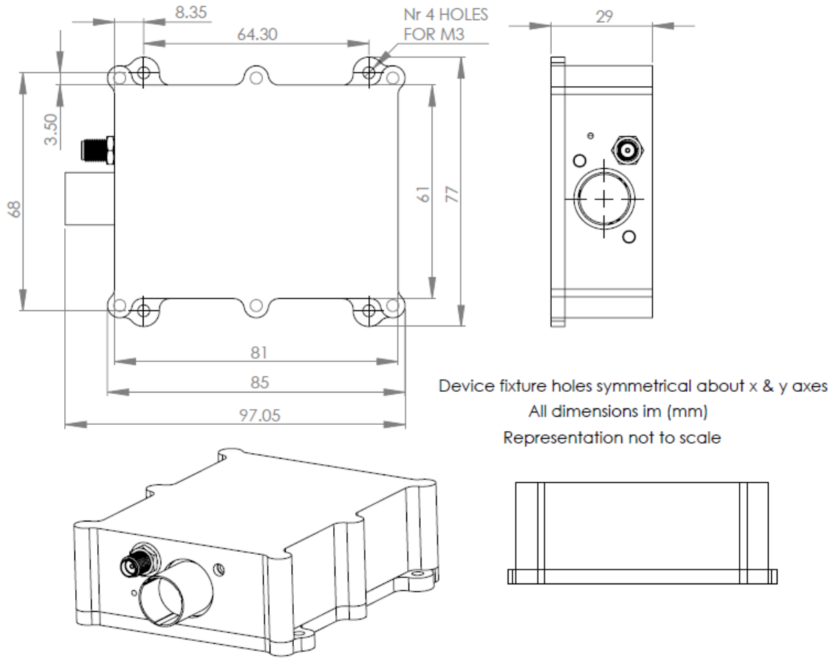
Figure 6 - ADR 4 Drawing
